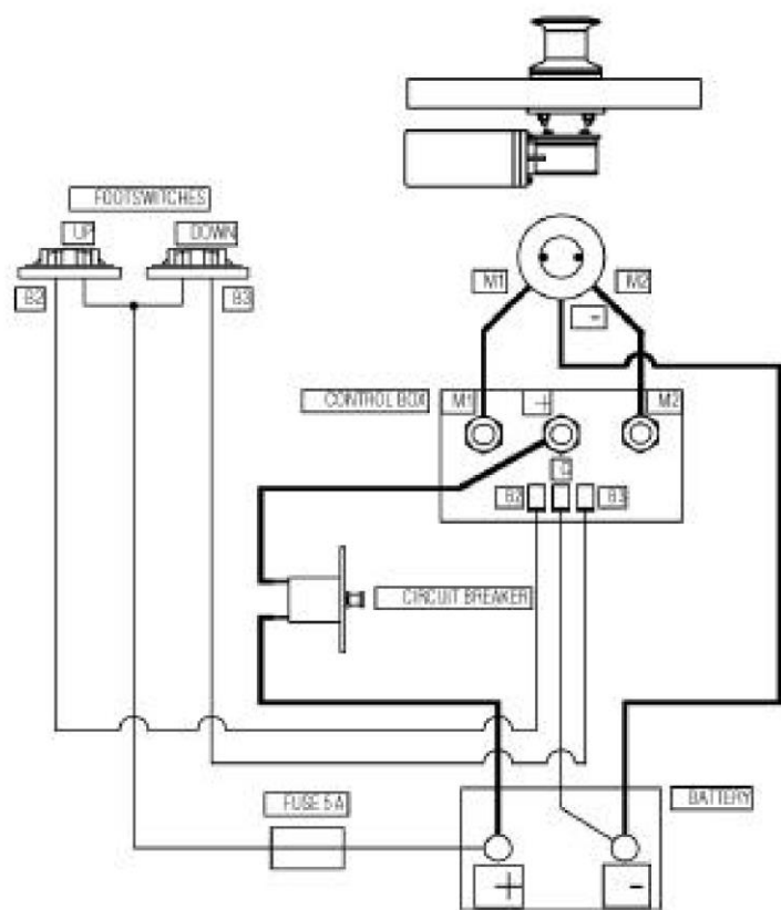
3 TERMINAL MOTORS
