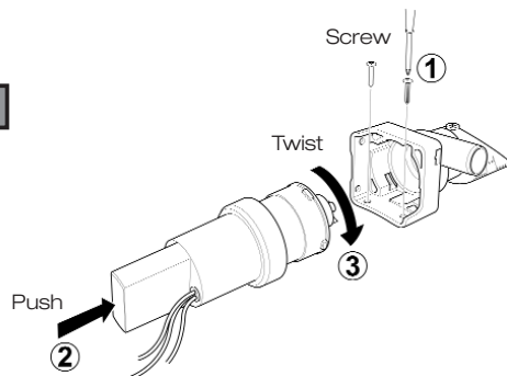
Figure 2- NOTE: Do NOT screw directly onto the hull
